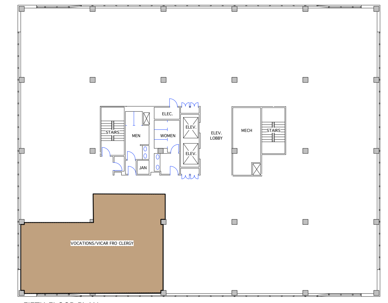
FIFTH FLOOR PLAN 1/8" = 1'-0"
