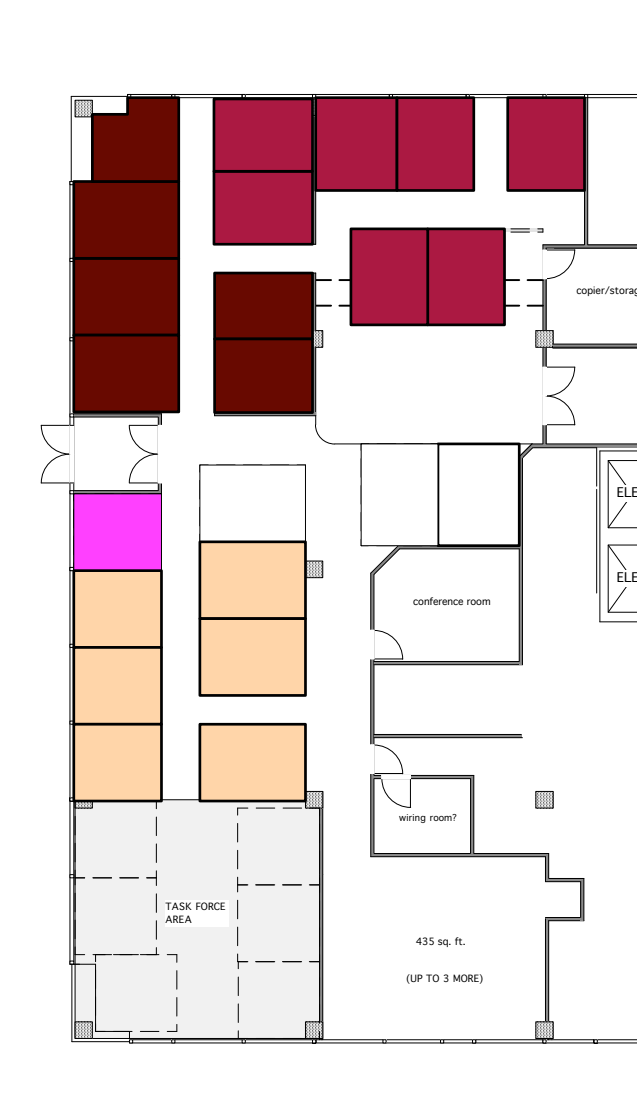
THIRD FLOOR PLAN 1/8" = 1'-0"
